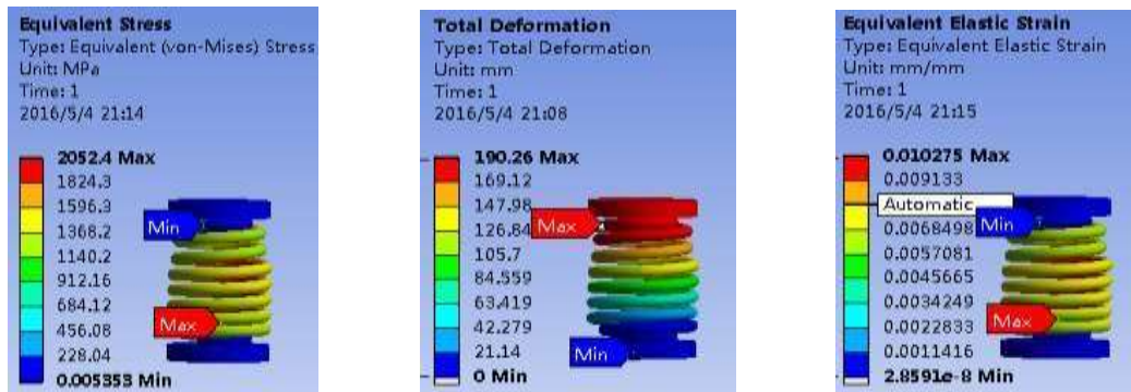
Fig13: Equivalent stress Fig14: Total deformation Fig15: Equivalent elastic strain Compression volume is 190mm
