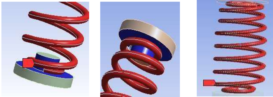
Fig3: endfrictionconstraint Fig4: Upperfrictionconstraint Fig5: self –contact
