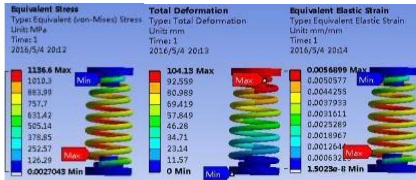
Fig10 Equivalent stress Fig11 Total deformation Fig12 Equivalent elastic strain Compression volume is 104mm
