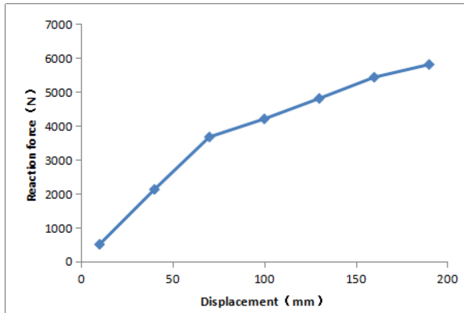
Fig16 :Displacement diagram
