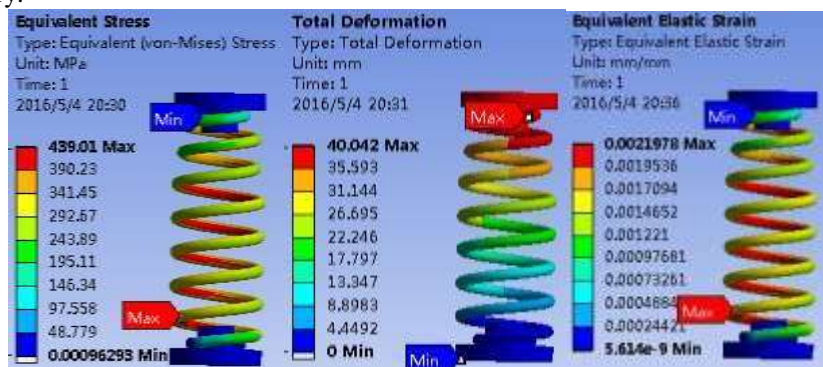
Fig7Equivalentstress Fig8Totaldeformation Fig9 Equivalent elasticstrain Compression volume is40mm
